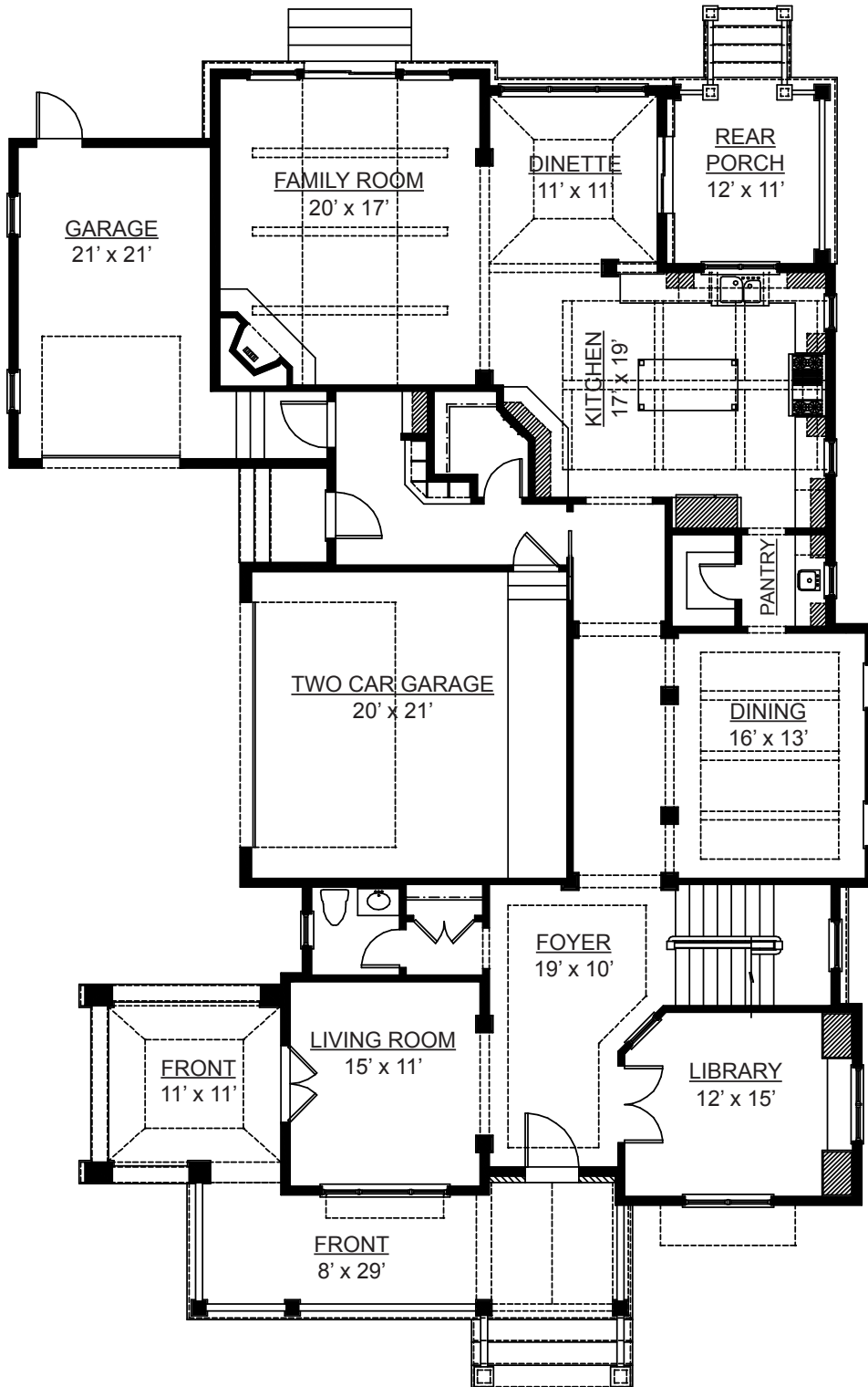
FIRST FLOOR PLAN (1,937 Square feet excluding garage)
